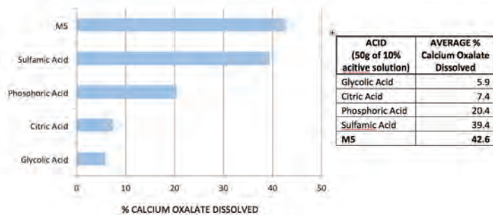
CALCIUM OXALATE DISSOLVING PROPERTIES OF ACIDS 5 MINUTE EXPOSURE (Recirculating Scale Removal)
